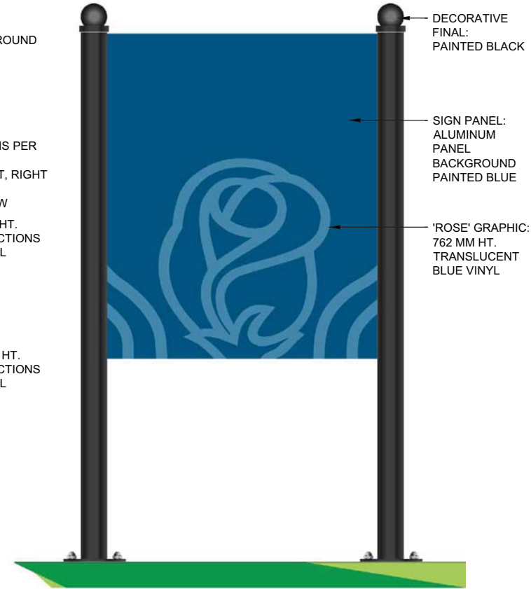
BACK ELEVATION
